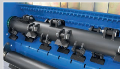
Controcoltelli dentati e supporto mazze dentato Notched counter-knives and notched hammer holder
